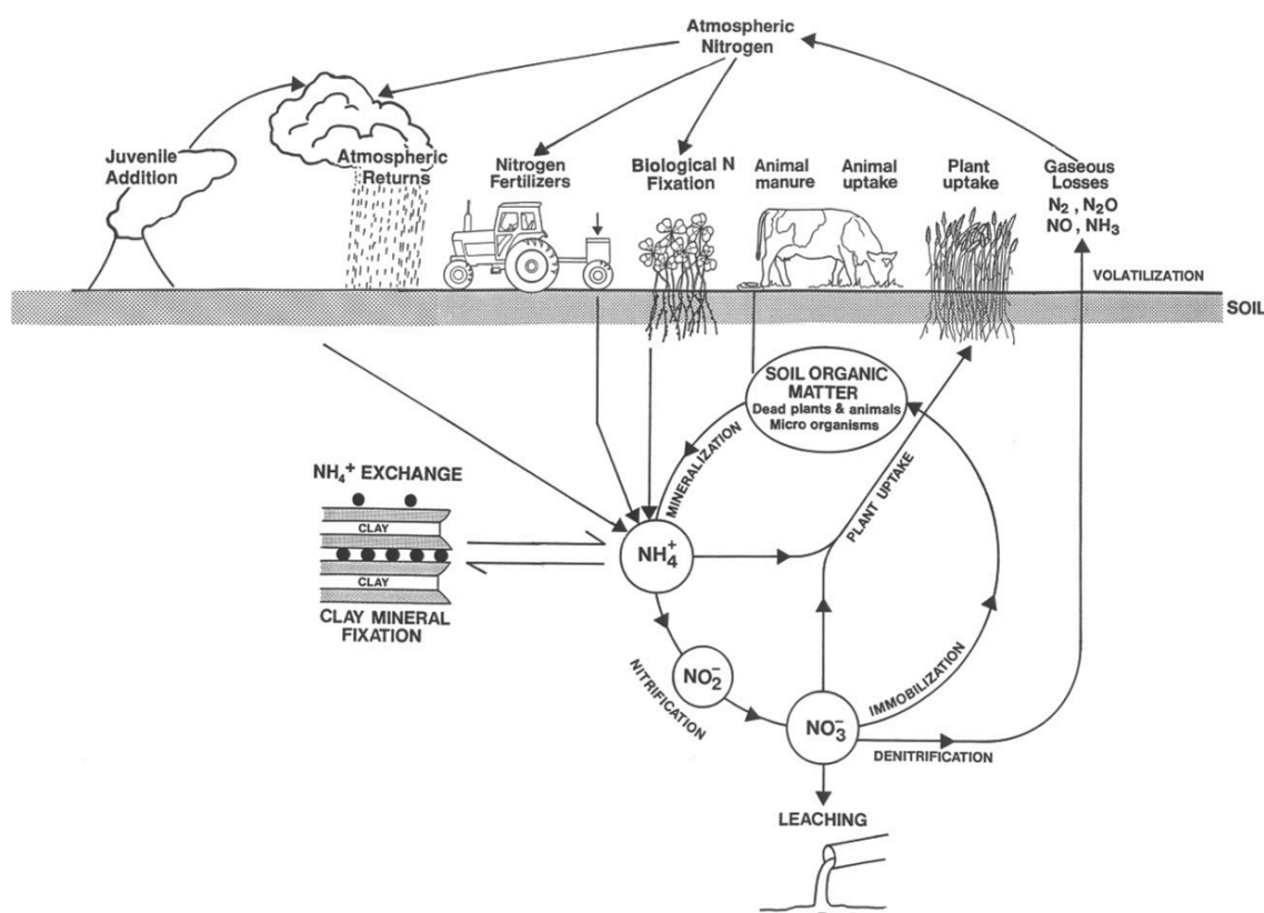
Figure 1. The nitrogen cycle for plant and soil in farming systems (from Cameron et al. 2013).
